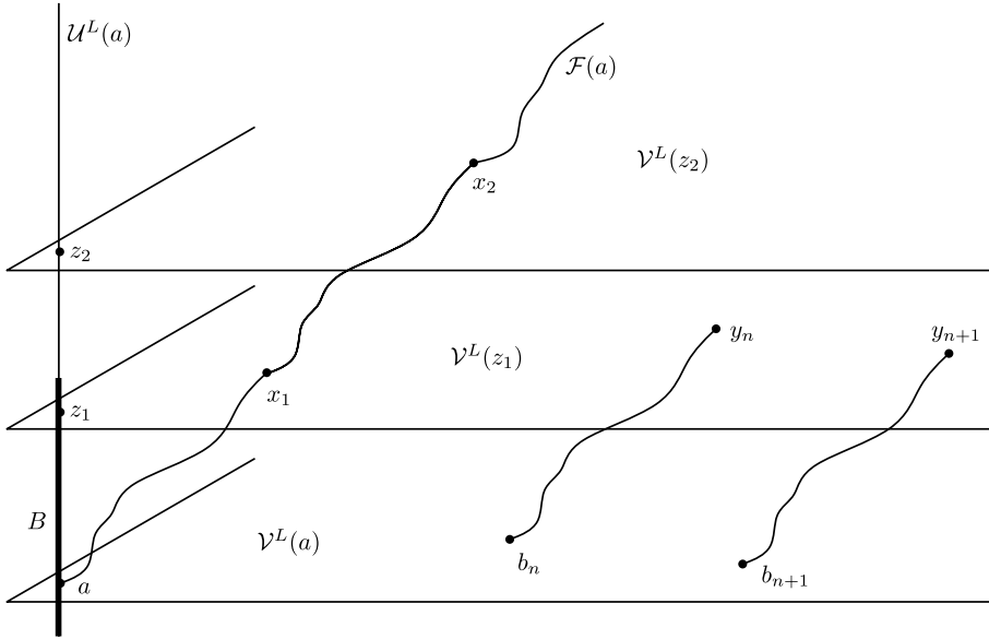
FIGURE 2. To the proof of Proposition 2.3.
