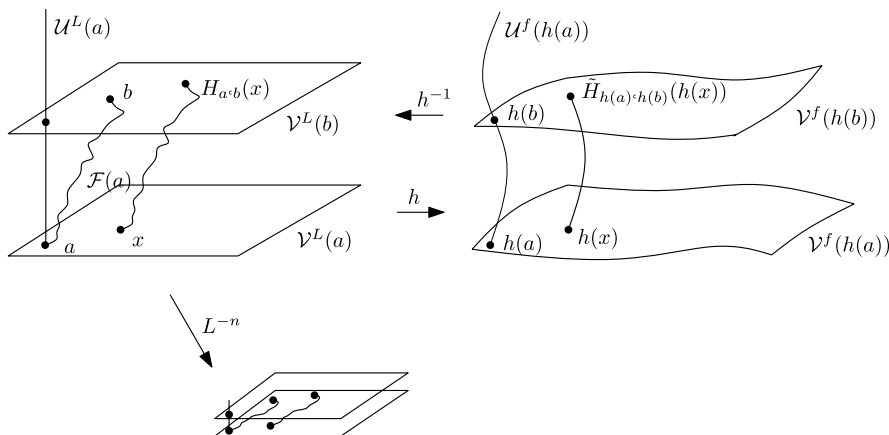
FIGURE 1. To the proof of Lemma 2.3.
